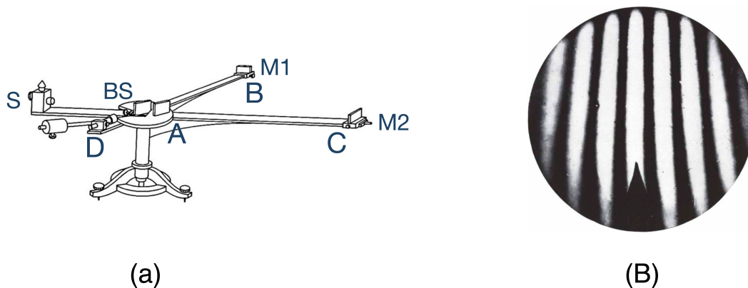
Figure 15.5: (A) On the left is a perspective engineering drawing of Michelson's prototype where I've labeled it like the sketch above. (B) On the right is a fringe pattern resulting from the apparatus (by the author).
