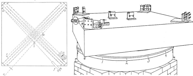
Figure 15.9: Plan and perspective engineering drawings of the Michelson Morley Experimental apparatus.
