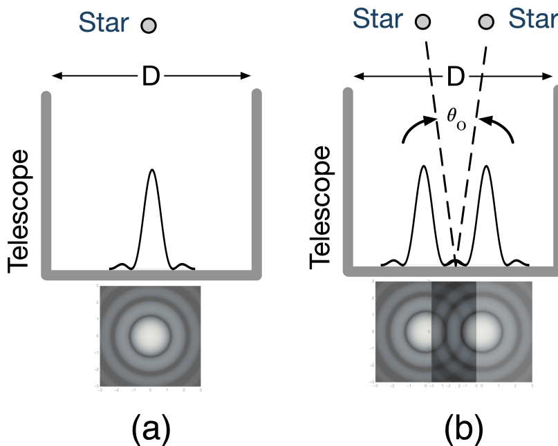
Figure 15.12: In (a) a single star is captured in a telescope of aperture D . The bullseye intensity pattern is shown at the bottom and the Intensity Curve is sketched at the receiving end (mirror) of the telescope. In (b) two stars are viewed with each creating its own intensity pattern, and overlapping Intensity Curves. The opening angle to the stars is shown as \theta_o .
