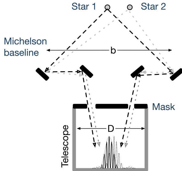
Figure 15.14: The Michelson design to increase the baseline beyond the edges of the Hooker Telescope. b = 3.07 m was the sweetspot.
