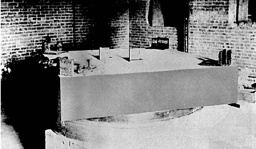
Figure 15.8: The Michelson-Morley apparatus on its huge concrete, rotating slab.
