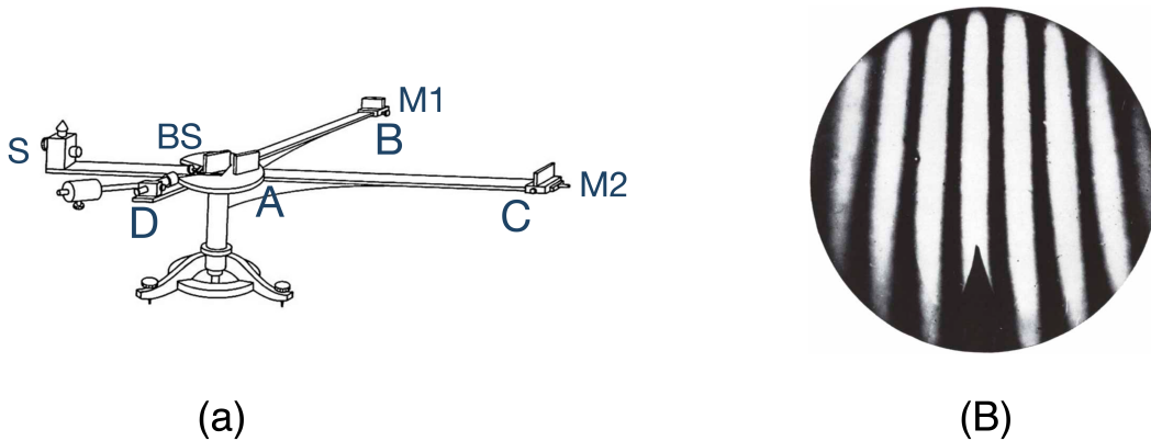
Figure 14.5: (A) On the left is a perspective engineering drawing of Michelson's prototype where I've labeled it like the sketch above. (B) On the right is a fringe pattern resulting from the apparatus (by the author).
